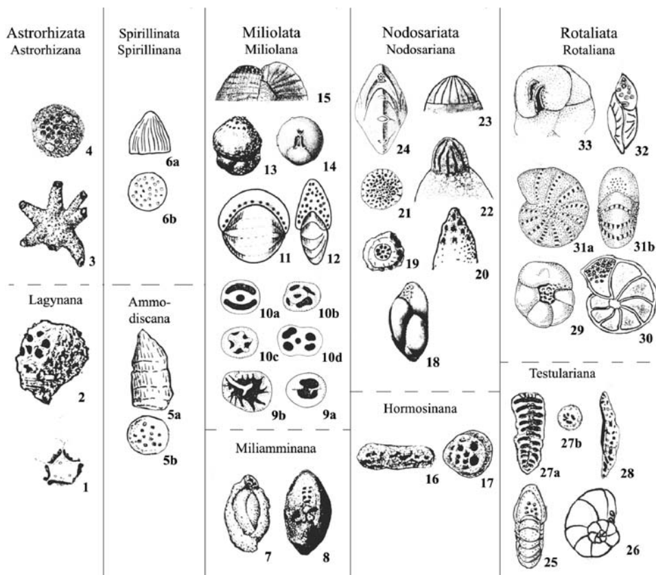
Fig. 6. Polymerization of apertures in different Foraminiferal classes. 1–4 – class Astrorhizata (1, 2 – subclass Lagynana, 3, 4 – subclass Astrorhizana), primary polymerized aperture: 1 – Microcometes , 2 – Guanduella , 3 – Astrorhiza , 4 – Orbulinelloides ; 5, 6 – class Spirillinata (5 – subclass Ammodiscana, 6 – subclass Spirillinana): 5a, b – Haurania , 6a, b – Ferayina ; 7–15 – class Miliolata (7, 8 – subclass Miliamminana, 9–15 – subclass Miliolana): 7 – Ammomassilina , 8 – Litola , 9a, b – polymerization of the inner teeth in Dentostomina , 10a–d – multiple aperture of Miliolids as a result of teeth fusion, 11 – Ovalveolina , 12 – Pseudedomia , 13 – Rhapydionina , 14 – Pyrgoella , 15 – Pseudohauerina ; 16–23 – class Nodosariata (16, 17 – subclass Hormosinana, 18 – 23 – subclass Nodosariana): 16 – Polychasmia , 17 – Cribratina , 18 – Delosina , 19 – Amphimorphina , 20 – Cribropleurostomella , 21 – Cribrolenticulina , 22 – Laevidentalina , 23 – Pandaglandulina , 24 – Cribrorobulina ; 25–33 – class Rotaliata (25–28 – subclass Textulariana, 29 – 33 – subclass Rotaliana): 25 – Cyclamina , 26 – Entzia , 27a, b – Cribrogoesella , a – section, b – apertural view, 28 – Poritextularia , 29 – Sesironophora , 30 – Anomalinella , 31a, b – Elphidium , 32 – Cribrorparrella , 33 – Anticleina (Cassidulinidae)
