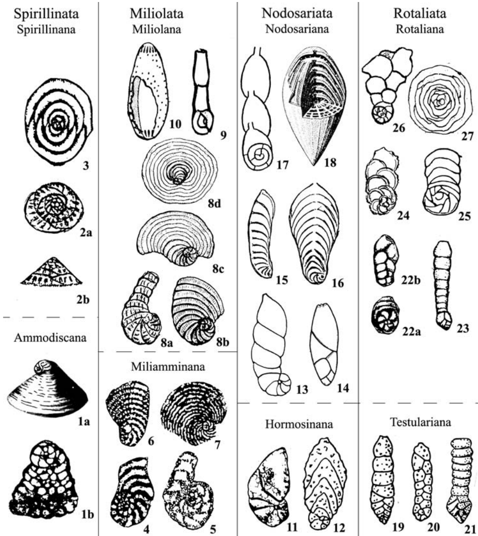
Fig. 5. Oligomerizations of the chambers in different foraminiferal classes. 1–3 – class Spirillinata (1 – subclass Ammodiscana , 2, 3 – subclass Spirillinana ): 1a, b – Coleiconus , b – section, 2a, b – Patellinella , 3 – Paleopatellina , five chambers in the initial whorl, two chambers in the last whorls; 4–10 – class Miliolata (4–7 – subclass Miliamminana , 8–10 – subclass Miliolana ): 4 – Feurtilia , 5 – Pseudocyclammina , 6 – Alzonella , 7 – Flabellocyclolina , 8a–d – different species of Peneroplis , 9 – Articularia , 10 – Idalina ; 11–18 – class Nodosariata (11, 12 – subclass Hormosinana , 13–18 – subclass Nodosariana ): 11 – Ammomarginulina , 12 – Flabellamina , 13 – Vaginulinopsis , 14 – Pyrulina , 15 – Astacolus , 16 – Palmula , 17 – Dimorphina , 18 – Colaniella ; 19–27 – class Rotaliata (19–21 – subclass Textulariana , 22–27 – subclass Rotaliana ): 19 – Bigenerina , 20 – Bolivinopsis , 21 – Clavulina , 22a, b – Caucasina , a – view of the initial trochospiral part, side view with the biserial last chambers, 23 – Rectobolivina , 24 – Siphonides , 25 – Rectoeponides , 26 – Dyocibicides , 27 – Cyclocibicides
